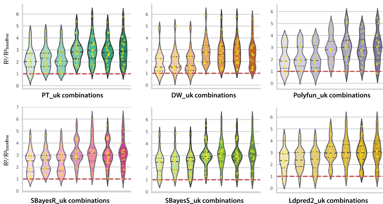
Figure 3. Prediction accuracy of PRS methods using the multiple-population strategy in the target population. (A) We used the Vietnamese height phenotype for the PRS model. The prediction accuracy was calculated based on multi-population training. The accuracy was measured as squared correlation ( R^2 ) between the true and predicted phenotypes in the testing dataset, averaged across 20-fold cross-validations for the whole genome except for chromosomes X and Y. The error bar indicates the standard deviation of R^2 across 20-fold. (B) Relative prediction accuracy of single and multi-population PRS using UKB combined with VN and JPN populations, with respect to the baseline models which is the average of PT and DW using 20-fold cross-validation in the Vietnamese population.
